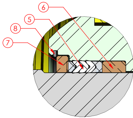
DETAIL B PACKING ORIENTATION
