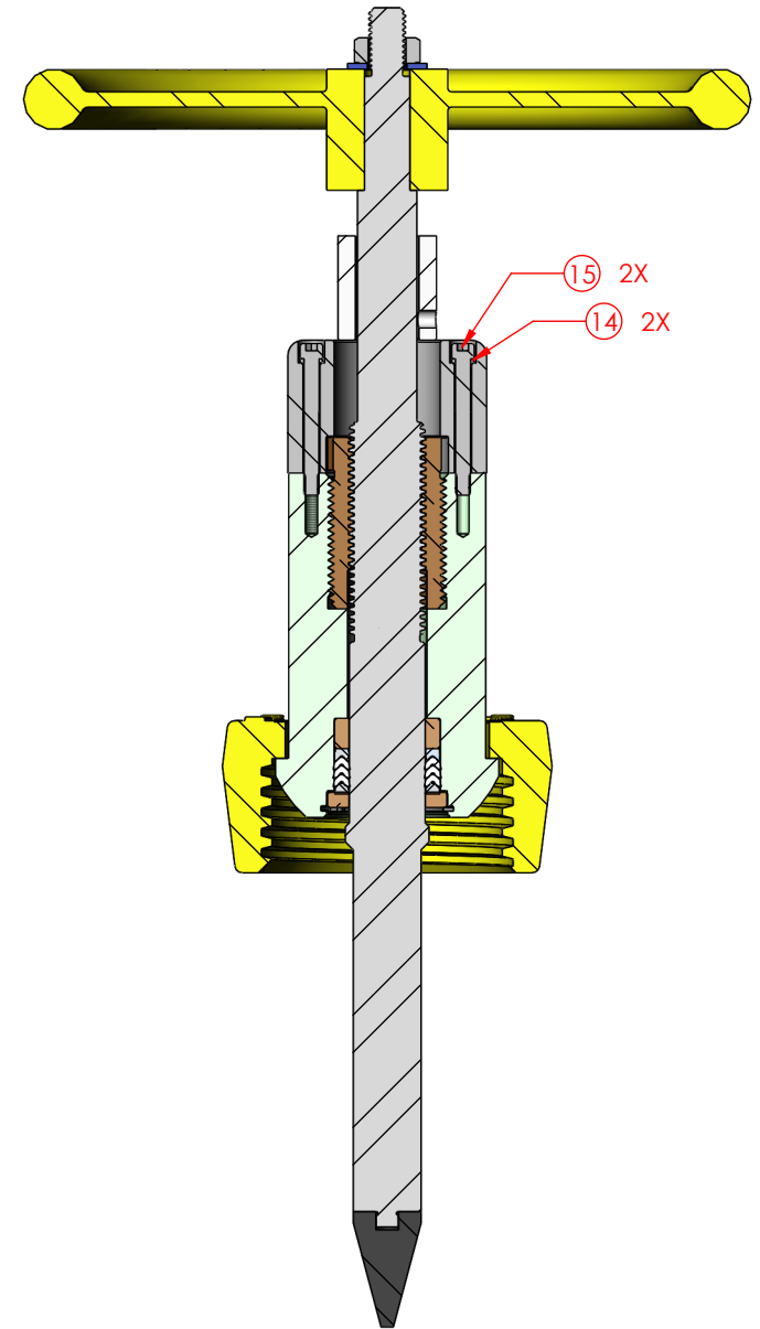
SECTION C-C
