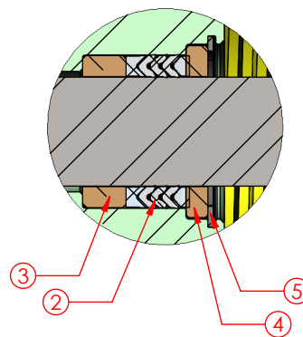
DETAIL A PACKING ORIENTATION
