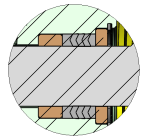
DETAIL A PACKING ORIENTATION
