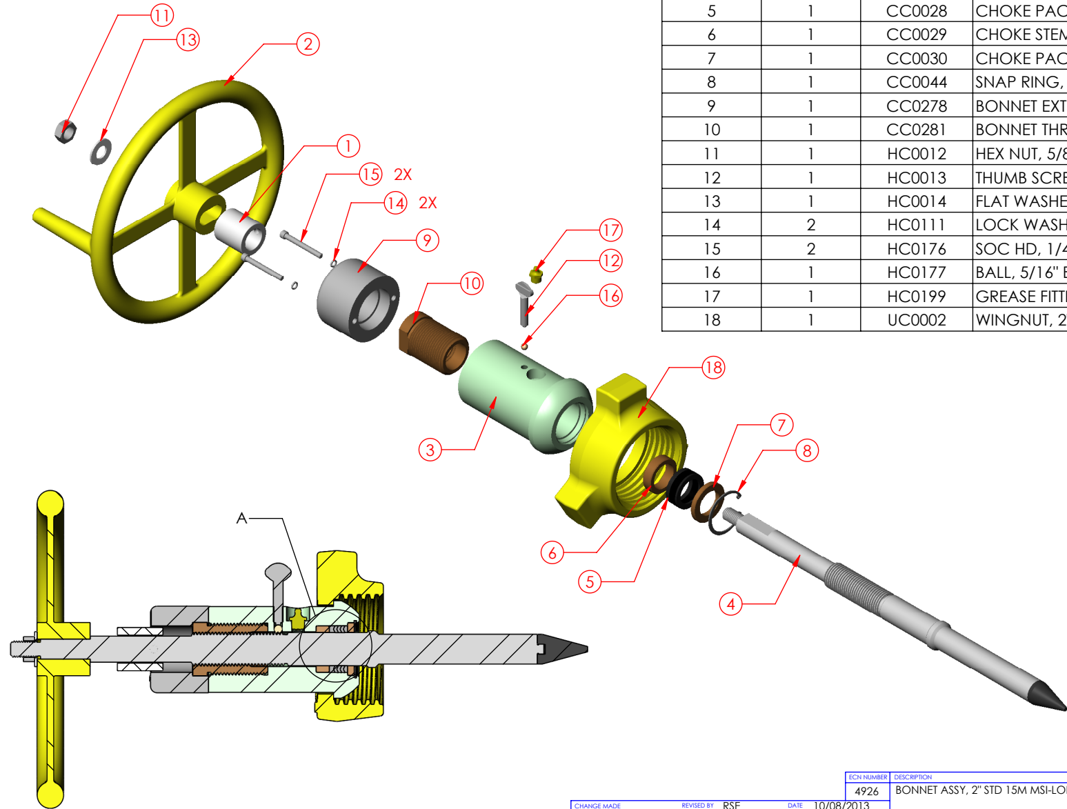
DETAIL A PACKING ORIENTATION
