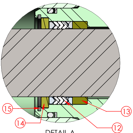
DETAIL A PACKING ORIENTATION
