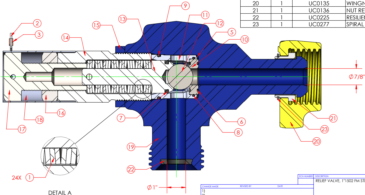
DETAIL A
